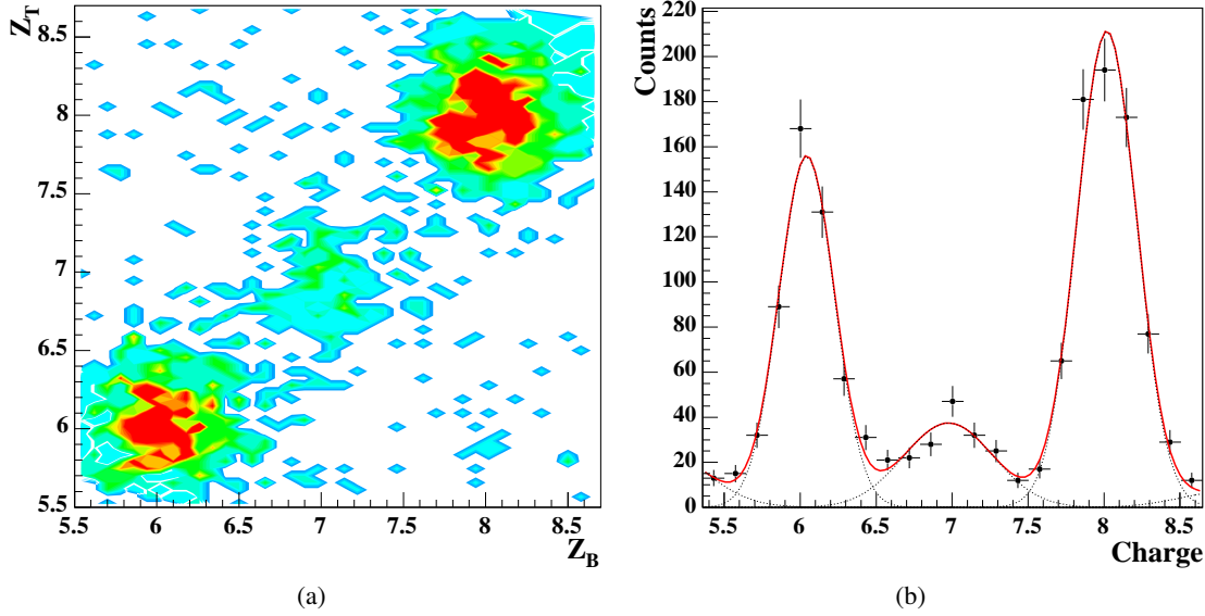
Figure 1: (a) Correlation between the reconstructed charge by the top ( Z_T ) and the bottom ( Z_B ) SCD planes. (b) Preliminary charge distribution of the CNO group with a superimposed multi-Gaussian function fit. The RMS values for C and O peaks from the fit are about 0.2e .
