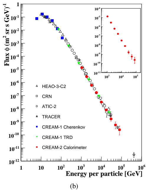
Figure 2: Cosmic-ray energy spectra for carbon (a) and oxygen (b) nuclei from HEAO [4], CRN [7], ATIC-2 [6] and TRACER [5] with preliminary results from the first [8] and second (red filled circles) flight of CREAM. The latter are also plotted separately in the inserts.
